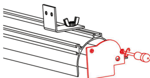
4. Insira as tampas finais
